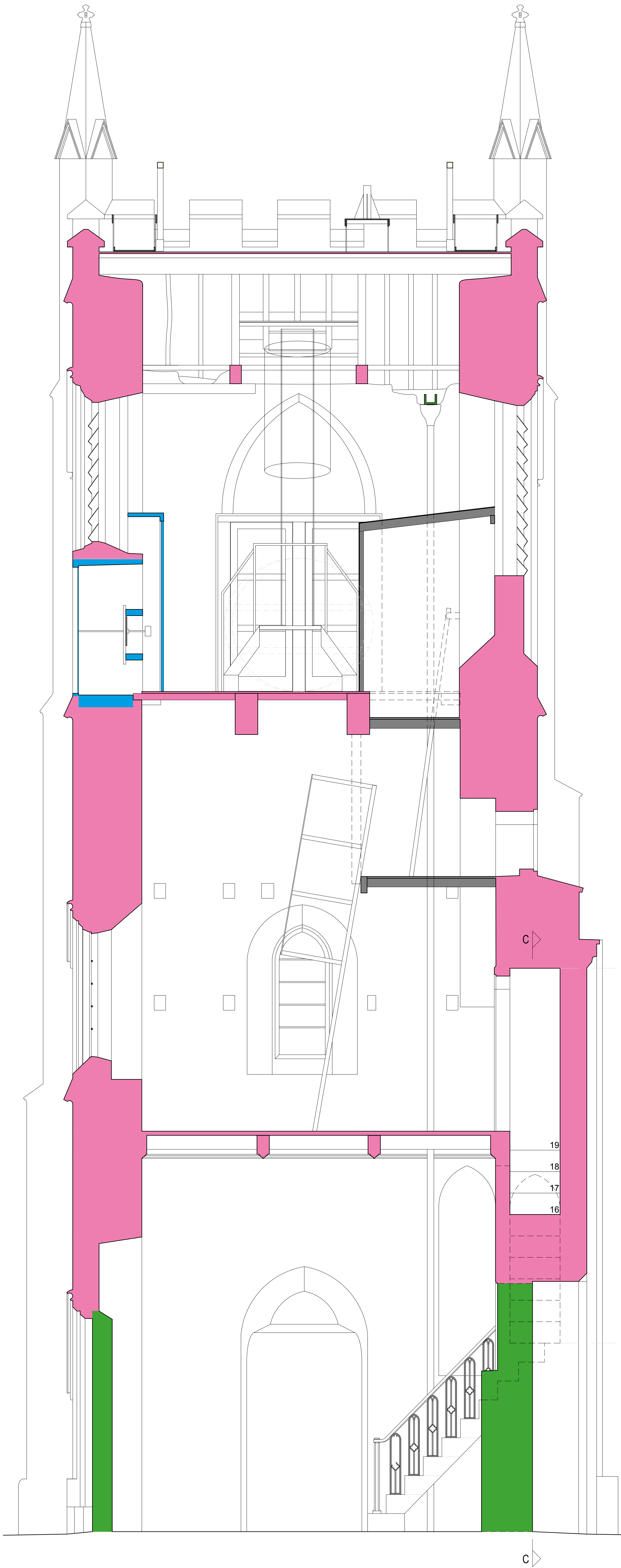
1 SECTION AA AS EXISTING 1:25
