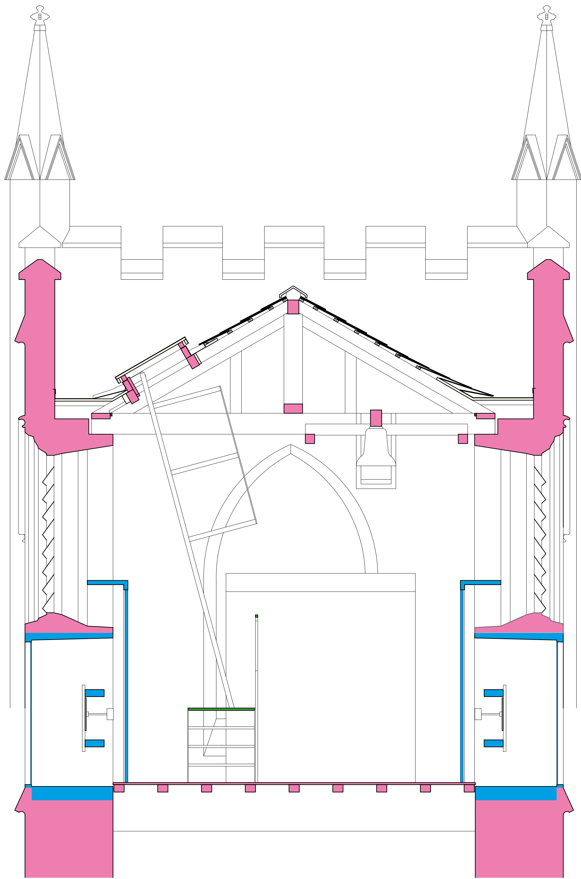
2 SECTION BB AS EXISTING 1:25
